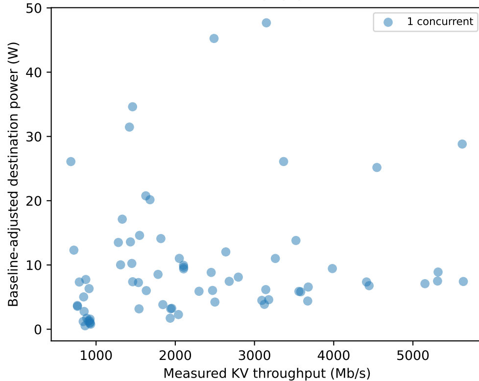
kv transfer
