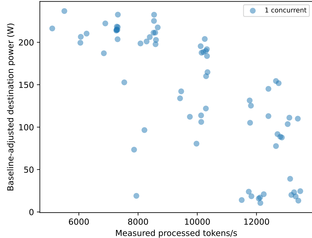
replay
