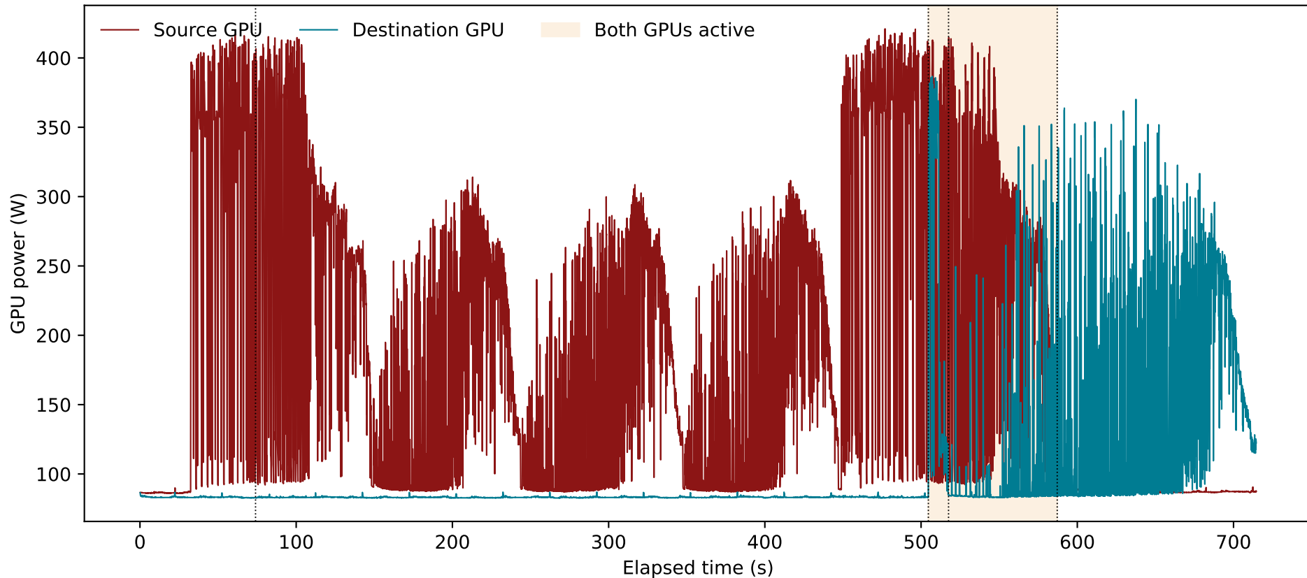
Queued replay migration: native 100 ms NVIDIA-SMI samples
