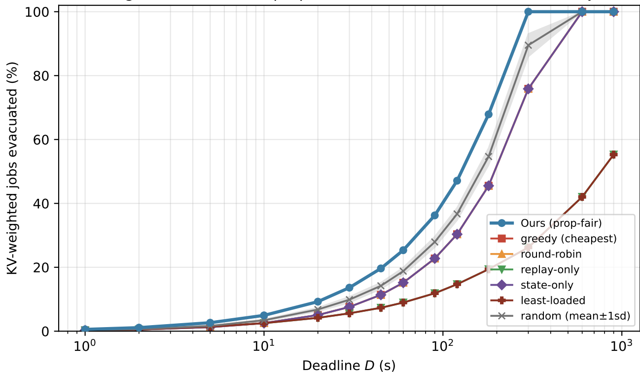
KV-weighted evacuation: proportional fairness vs. baselines (10k jobs)
