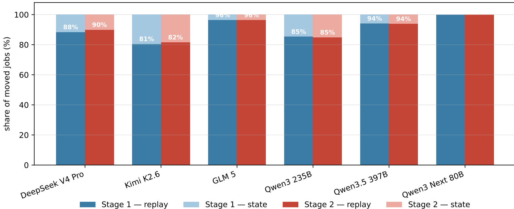
Per-model action mix: Stage 1 vs Stage 2 replay (dark) / state-transfer (light); \phi^* = 0.9256
