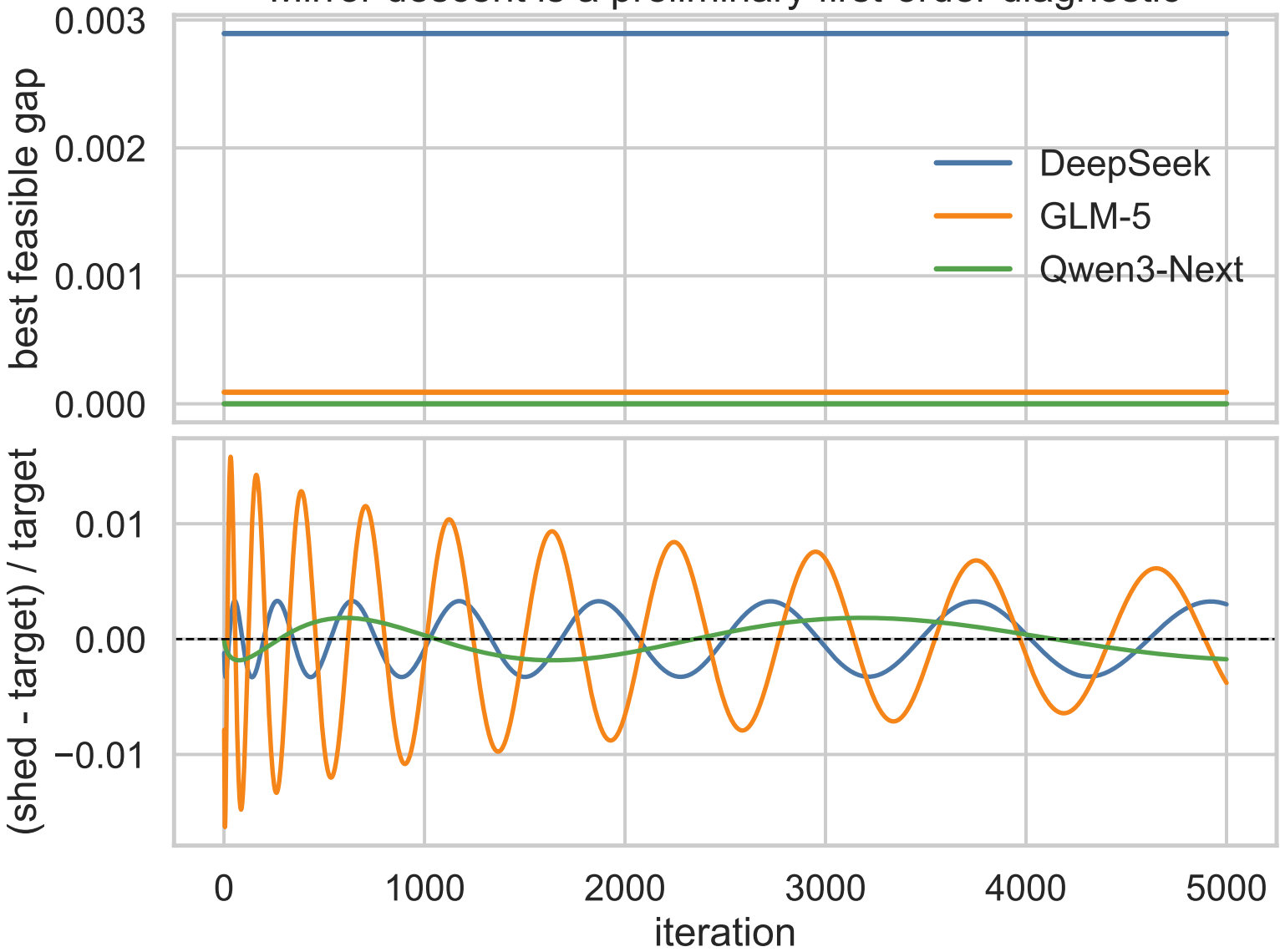
Mirror descent is a preliminary first-order diagnostic
