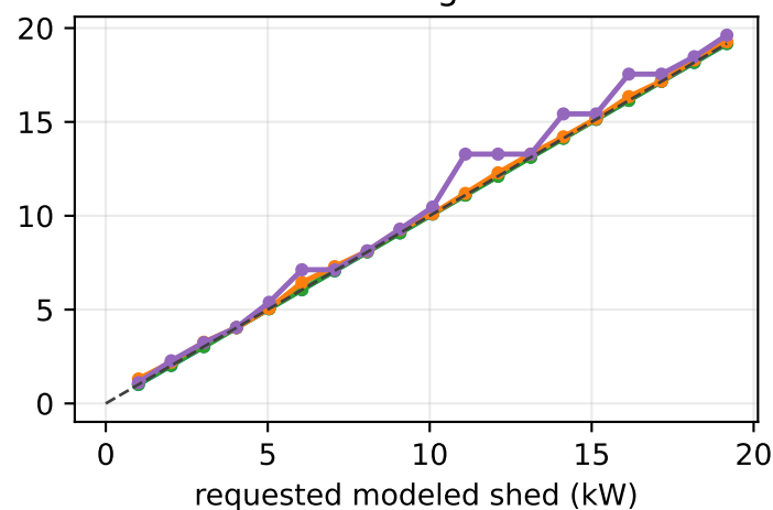
reasoning chat
