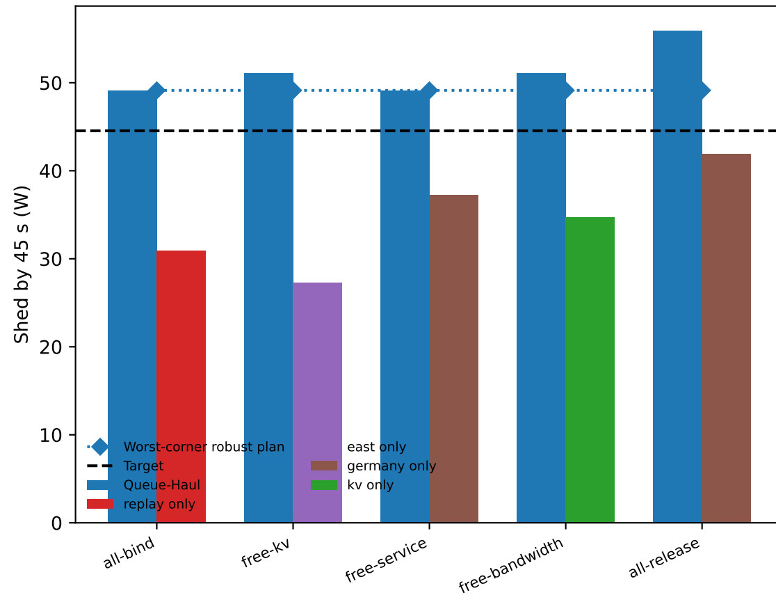
One-at-a-time releases
