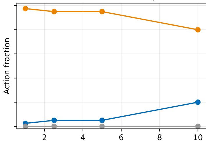
Queue-Haul Greedy
