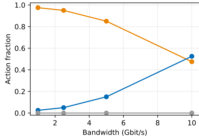
Queue-Haul LP
