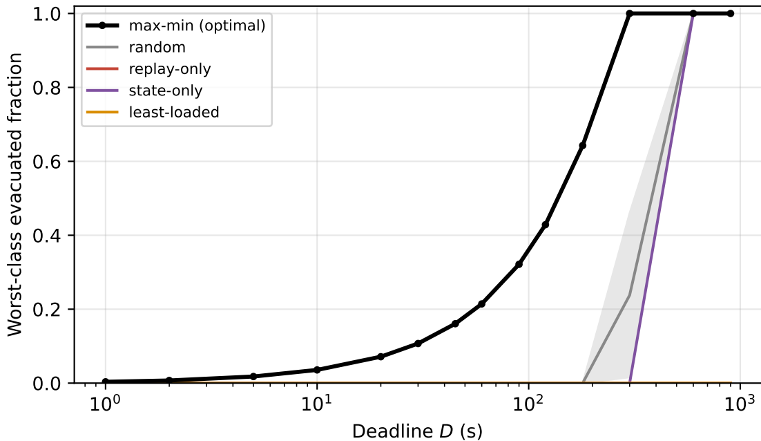
Worst-class protection: optimizer vs baselines
