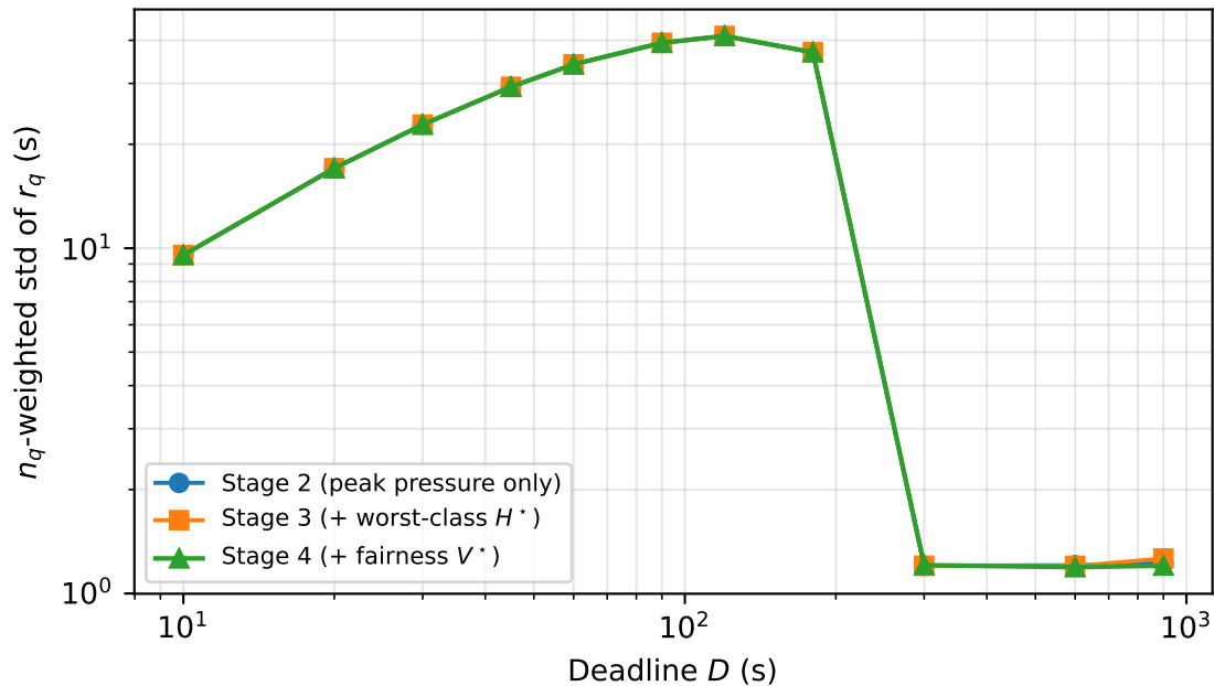
Spread of per-class reconstruction cost vs D (10,000 jobs)
