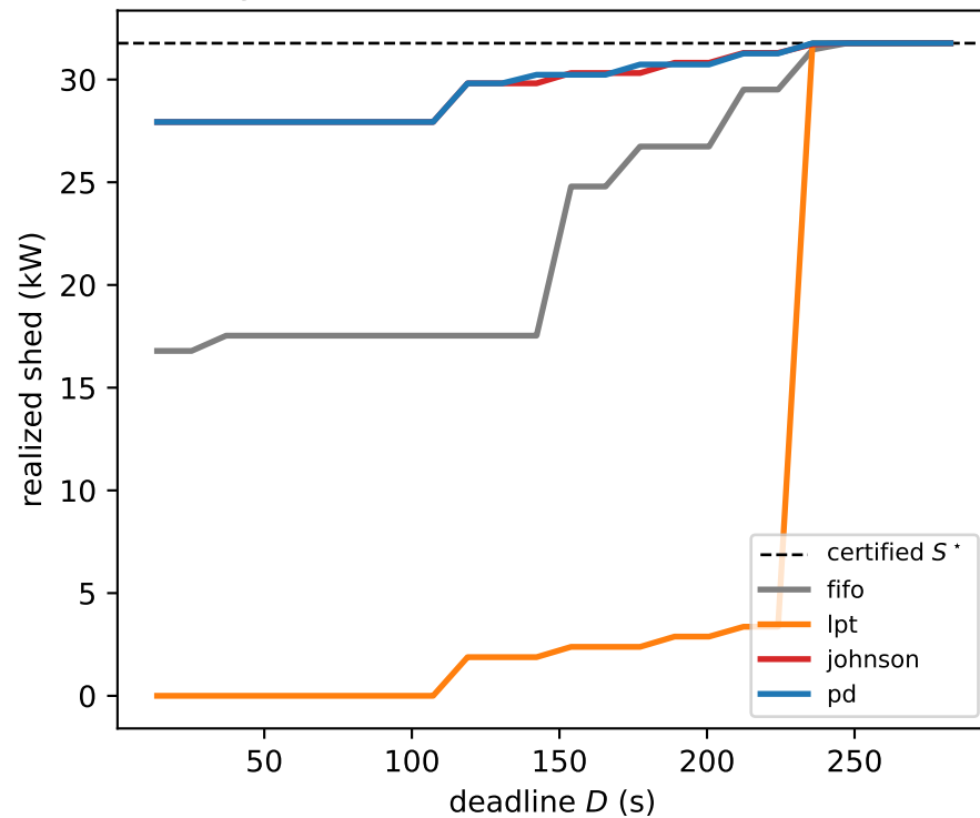
A · grid relief: order-blindness wastes shed
