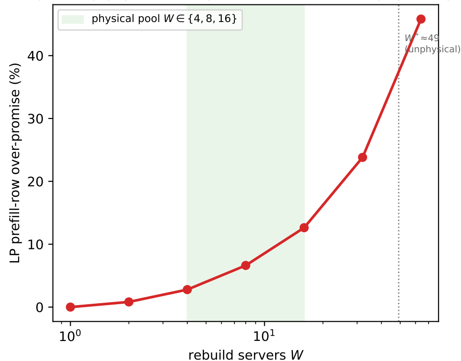
B · packing gap: LP over-promises even in the physical pool
