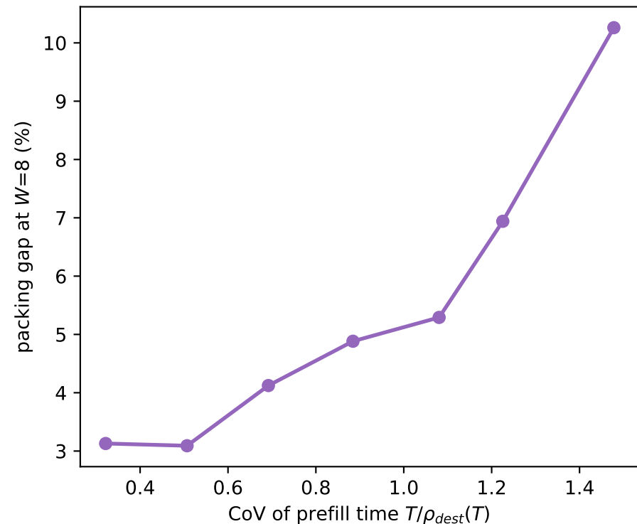
C · tail heaviness worsens the gap at physical W=8
