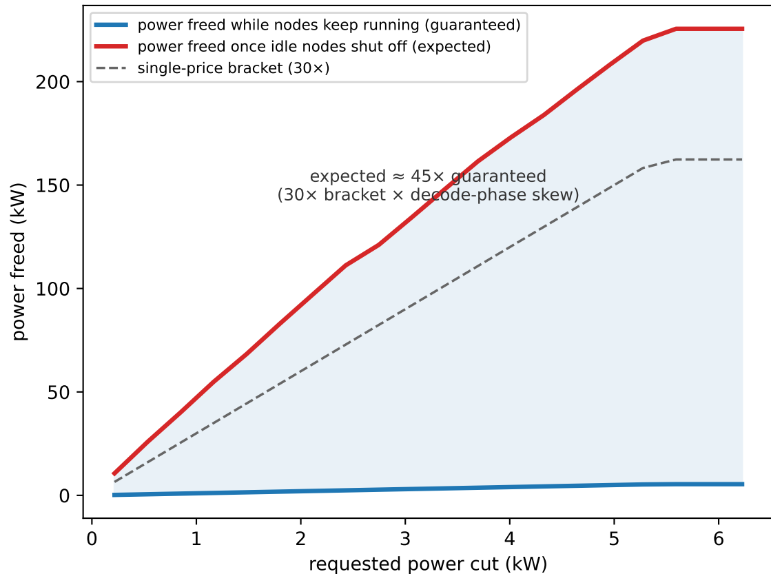
Compute-bound pool: certified floor far below expected power freed
