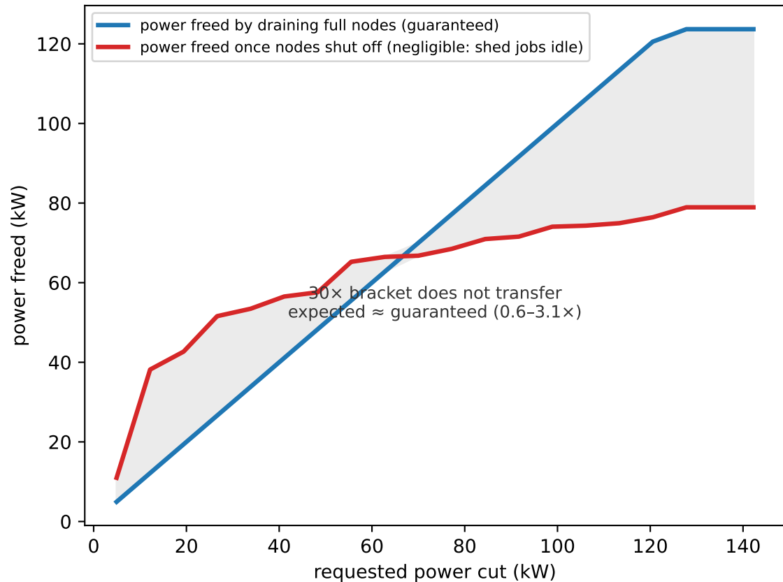
Memory-bound pool: shut-off saving absent, expected \approx guaranteed
