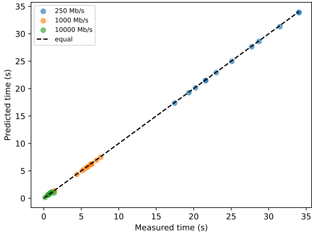
kv transfer
