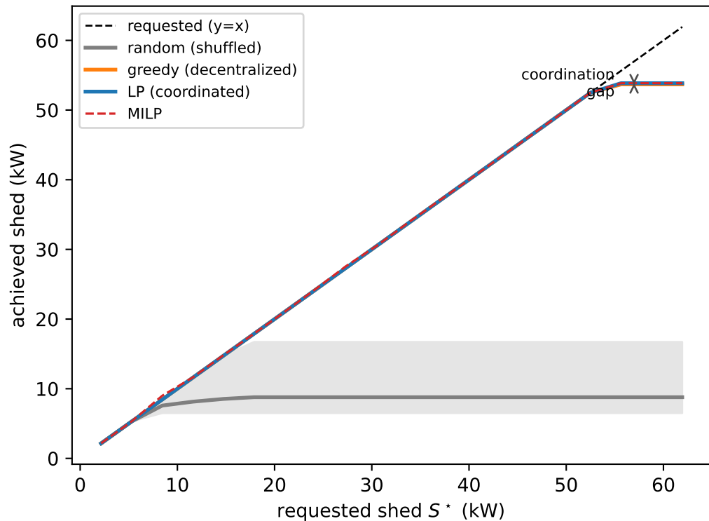
random < greedy < LP: selection then coordination
