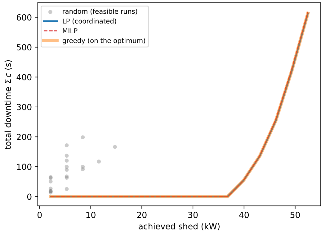
random pays more per watt; greedy = LP optimum where feasible
