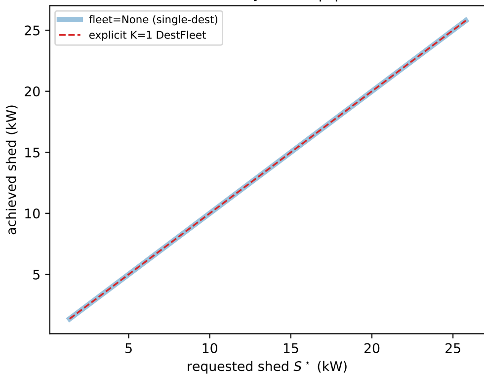
A. K=1 reduces exactly ( \max |\Delta| = 0.0e+00 W)
