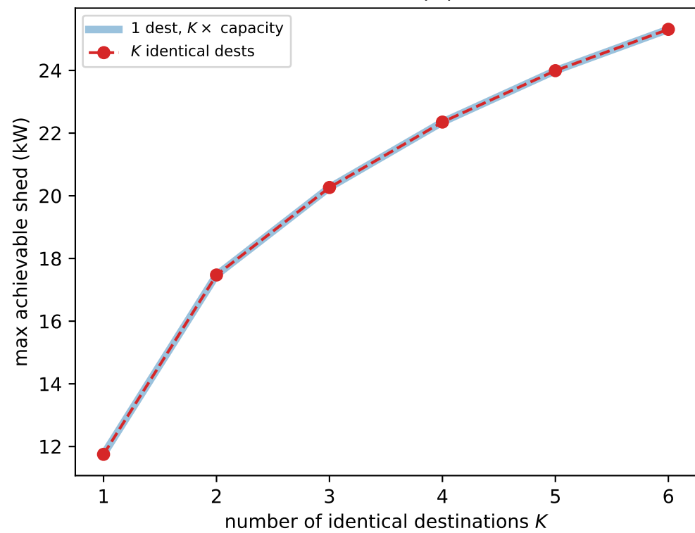
B. split \equiv merged ( \max |\Delta| = 0.0e+00 kW)
