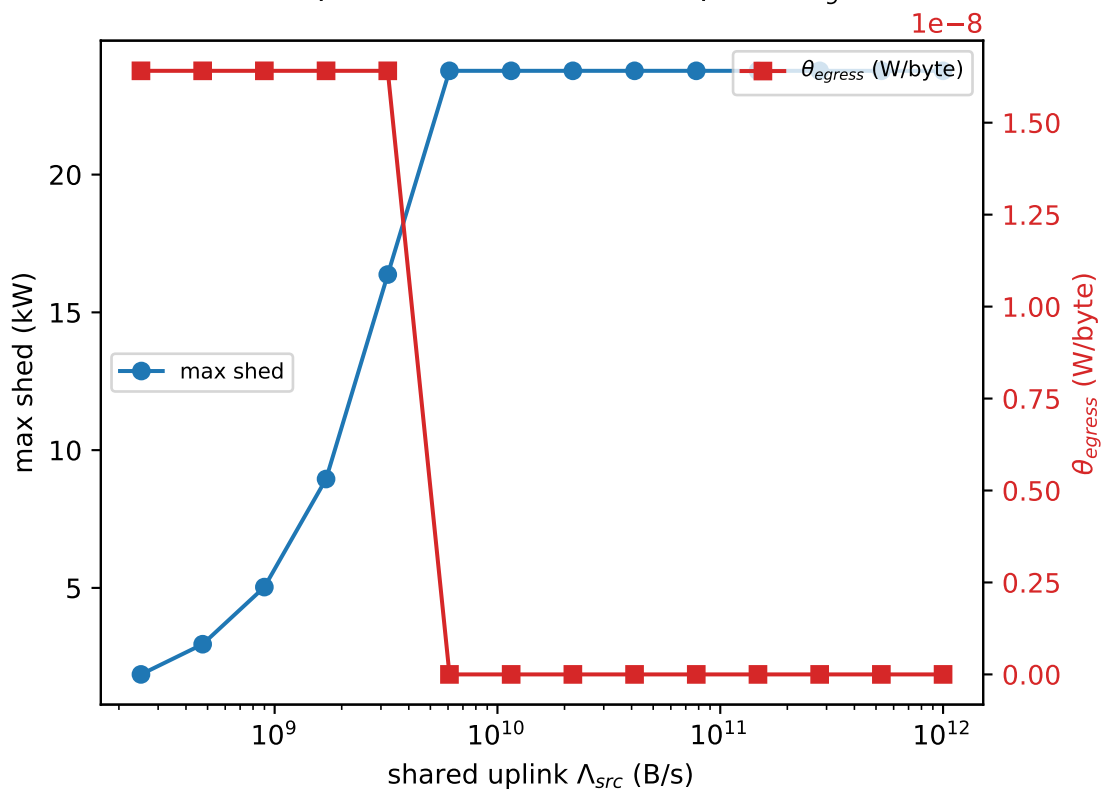
C. shared uplink binds \rightarrow shed collapses, \theta_{egress} > 0
