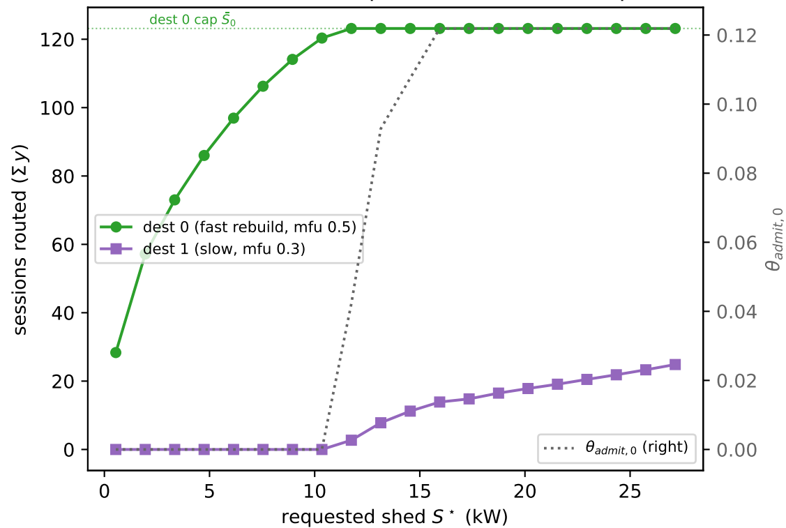
D. concentrate on cheapest-reachable, then spread
