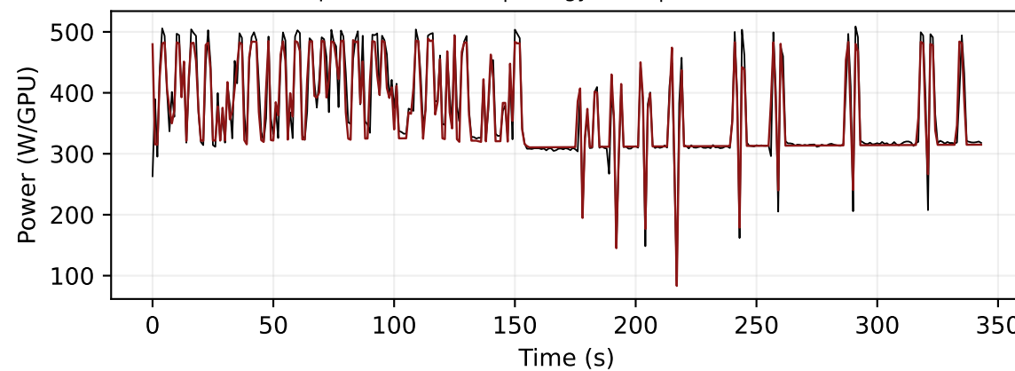
pack 2 cache-off | energy 0.6% | NRMSE 0.058
