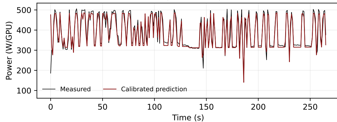
pack 1 cache-off | energy 1.3% | NRMSE 0.095
