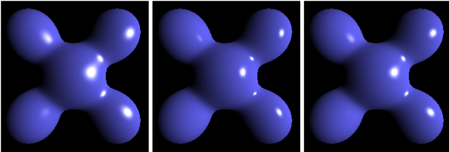
Blinn-Phong
