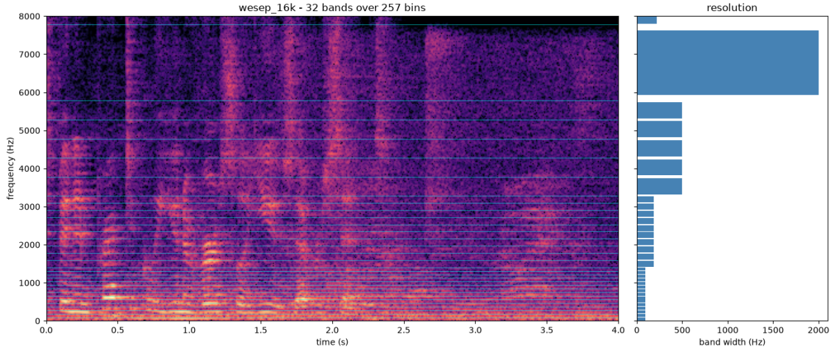
Figure 3.3: The band plan used here, shown against a four-second mixture from the training set. Left: the band boundaries drawn over the spectrogram, closely spaced at the bottom where the speech structure is and widening upwards. Right: the width of each band in hertz.
