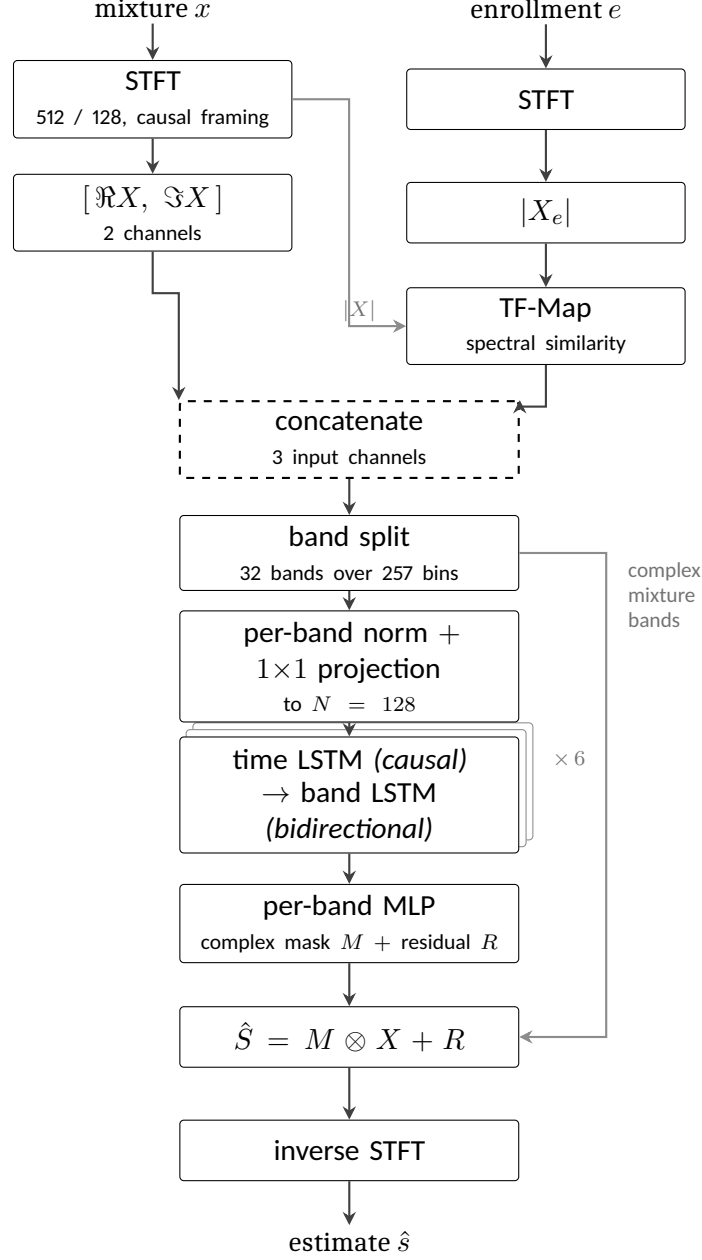
Figure 3.2: The extractor as implemented. Band splitting and the interleaved band-level and sequence-level modelling follow [7]; the mask-plus-residual estimator follows [8]; TF-Map conditioning follows [27]. The causal time path and the third input channel are this work's.
