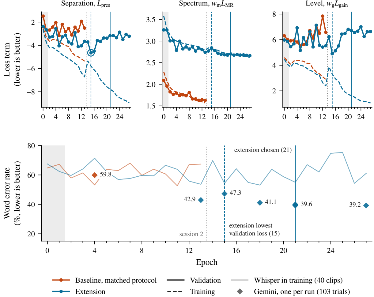
Figure 4.1: Training (dashed) and validation (solid) scores per epoch, counted from zero, for the baseline (orange) and the extension (blue), trained under the same protocol: the in-training Whisper check sets the learning rate and decides which epochs are kept. The baseline shown is epochs 0–13 of a 28-epoch run and is not yet judged; it is not the earlier baseline run that gives epoch 6 in the results tables. Top: the three weighted terms of the target-present loss, the first bracket of Equation 3.11, which add up to it (lower is better): separation L_{\text{pres}} , spectrum w_m L_{\text{MR}} and level w_g L_{\text{gain}} . Bottom: word error rate on the 103 validation trials with both speakers present (lower is better). Each diamond is one run of the live judge on the same audio, labelled with the mean of the runs at that epoch; the thin lines are the in-training Whisper small.en check on 40 validation clips. Shaded epochs fail the -10 dB silence bar in both runs. The solid vertical line marks the extension’s chosen epoch, the dashed one its lowest validation loss (the sum of the three terms), and the grey dotted line where training resumed in a second session.
