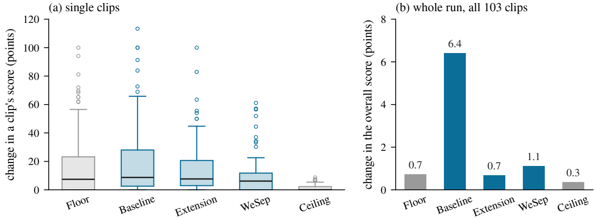
Figure 5.1: How much Gemini’s LCF-WER changed across the three runs in Table 5.2, where change is the highest of the three run scores minus the lowest. (a) The box plot showing how the change varies per clip over the averaged runs. A clip’s score can pass 100 % and can occur when Gemini adds words through hallucination or by including interfering speech. (b) Change in the overall score over all 103 clips. Floor and ceiling (grey) are reference points.
