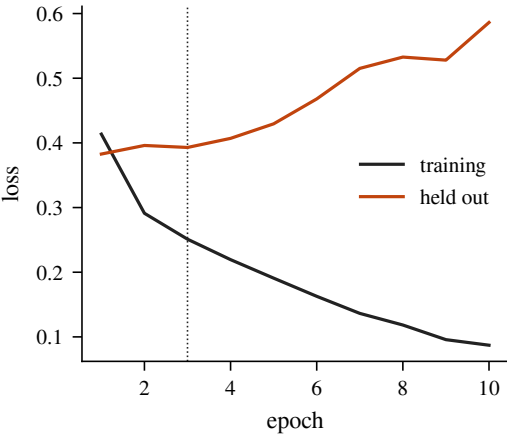
Training loss falls; held-out loss turns
