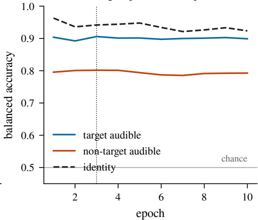
Nothing improves after epoch 3
