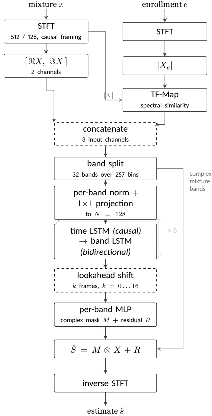
Figure 3.3: The extractor as implemented. Band splitting and the interleaved band-level and sequence-level modelling follow [5]; the mask-plus-residual estimator follows [6]; TF-Map conditioning follows [19]. The causal time path, the lookahead shift and the third input channel are this work's.
