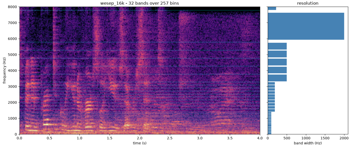
Figure 3.3: The band plan used here, shown against a four-second mixture from the training set. Left: the band boundaries drawn over the spectrogram, closely spaced at the bottom where the speech structure is and widening upwards. Right: the width of each band in hertz.
