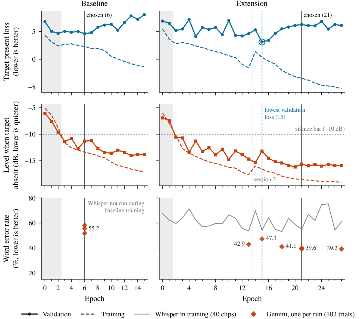
Figure 4.1: Training (dashed) and validation (solid) scores per epoch, counted from zero, for the baseline (left) and the extension (right). Top: target-present loss, the first bracket of Equation 3.12 (lower is better). Middle: output level on target-absent clips relative to the mixture, L_{\text{abs}} (lower is quieter); the dotted line is the -10 dB silence bar, and shaded epochs fail it. Bottom: word error rate on the 103 validation trials with both speakers present (lower is better). Each diamond is one run of the live judge on the same audio, labelled with the mean of the runs at that epoch; the grey line is the in-training Whisper small.en check on 40 validation clips, which was not run for the baseline. The solid vertical line marks the chosen epoch, the blue dashed line the extension’s lowest validation loss, and the grey dotted line where the extension’s training resumed in a second session.
