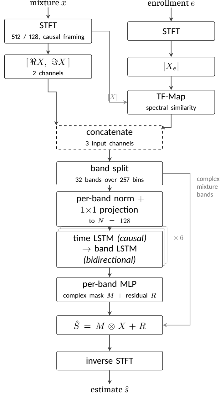
Figure 3.3: The extractor as implemented. Band splitting and the interleaved band-level and sequence-level modelling follow [5]; the mask-plus-residual estimator follows [6]; TF-Map conditioning follows [19]. The causal time path and the third input channel are this work’s.
