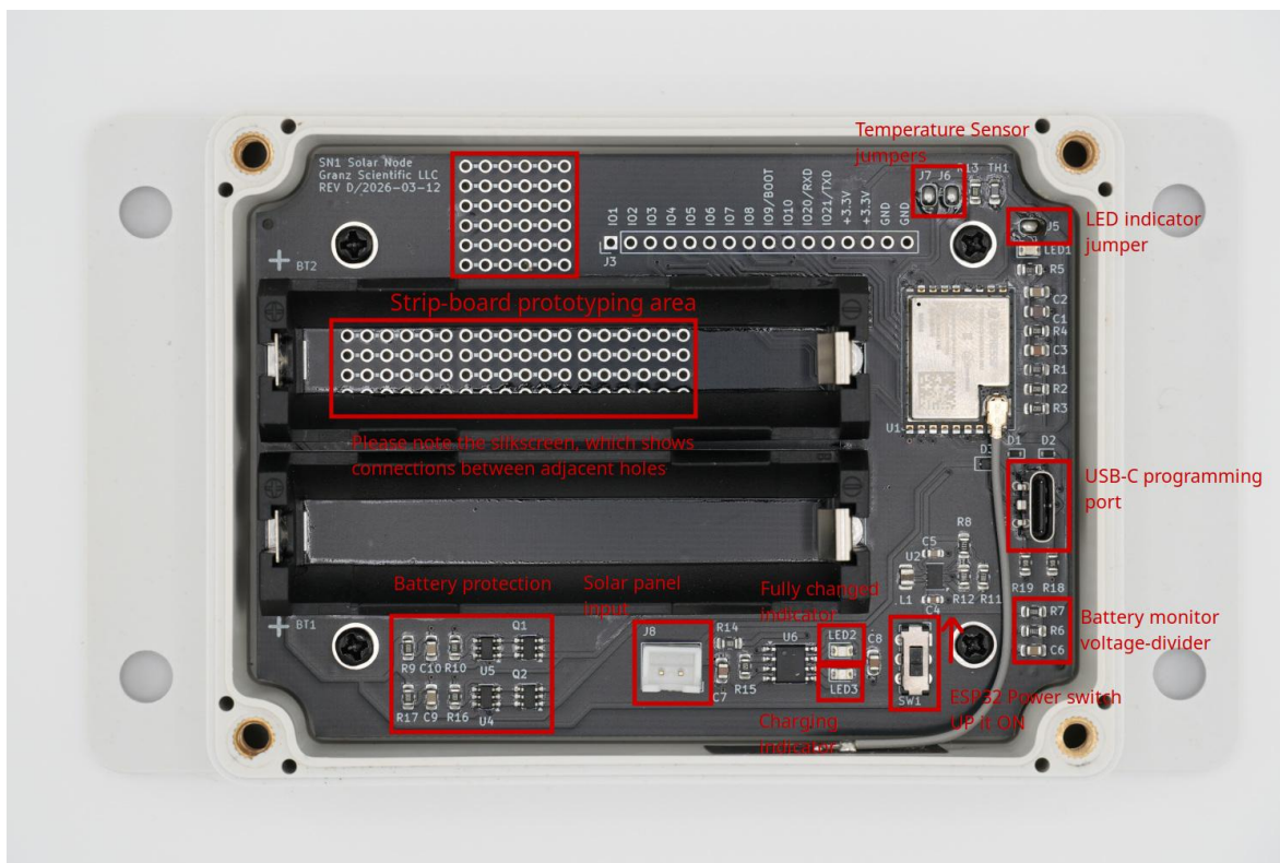
Figure 3: System Layout
