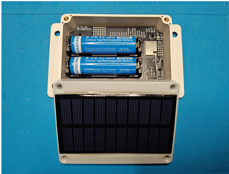
Figure 1: SN1 Solar Node
