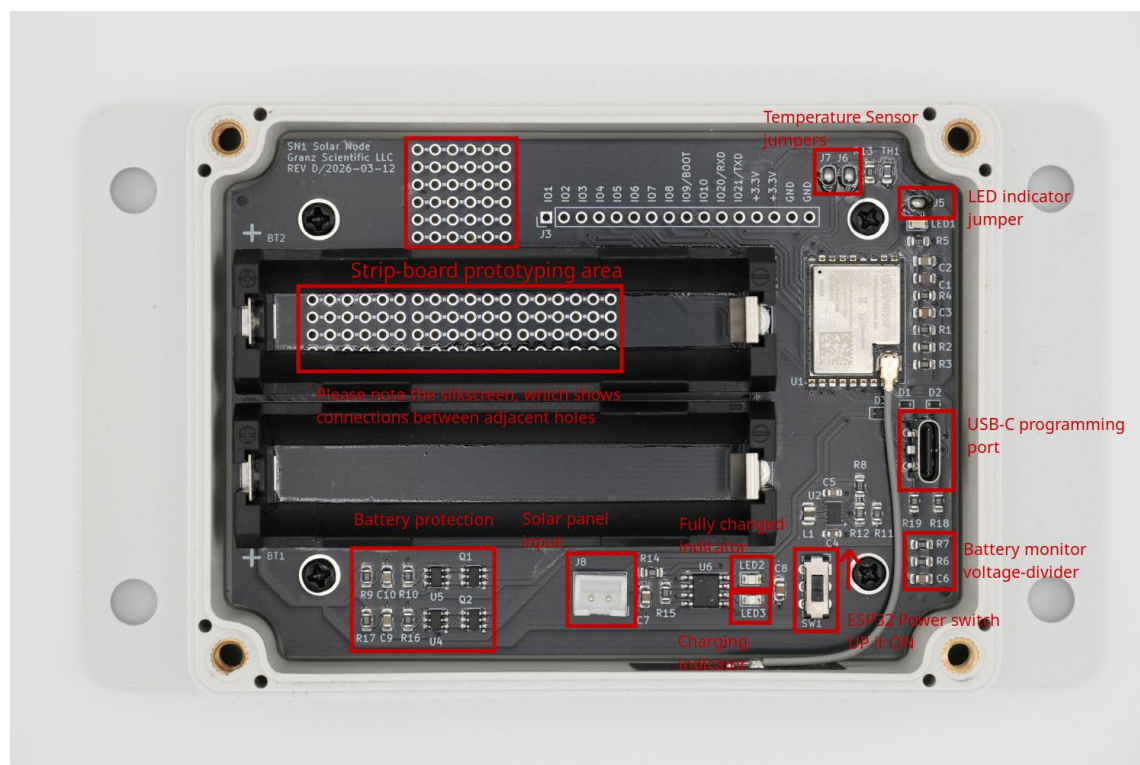
Figure 3: System Layout
