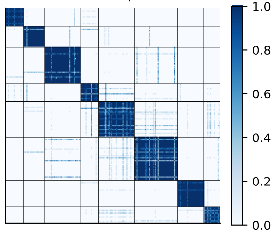
Co-association matrix, consensus k=8
