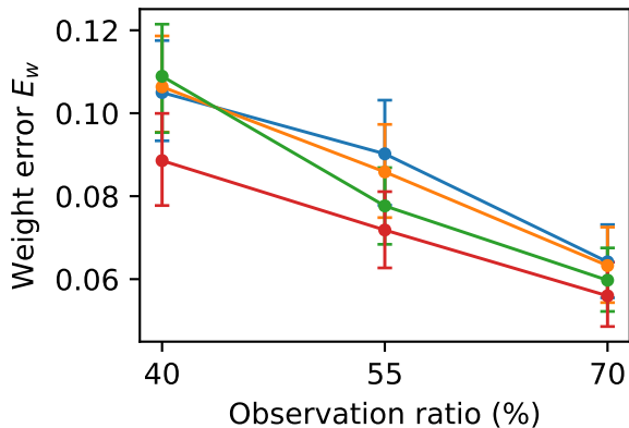
(c) Weight error E_w
