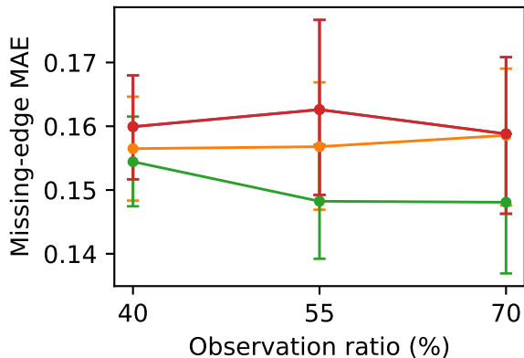
(a) Missing-edge MAE
