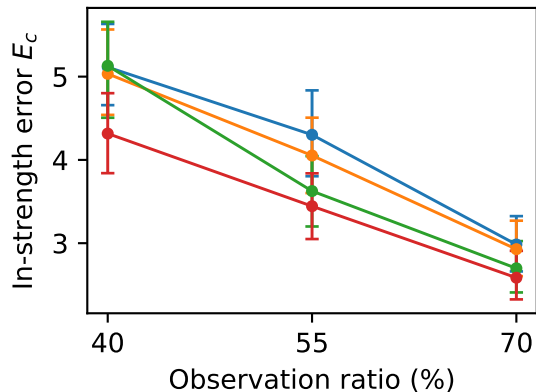
(b) In-strength error E_c
