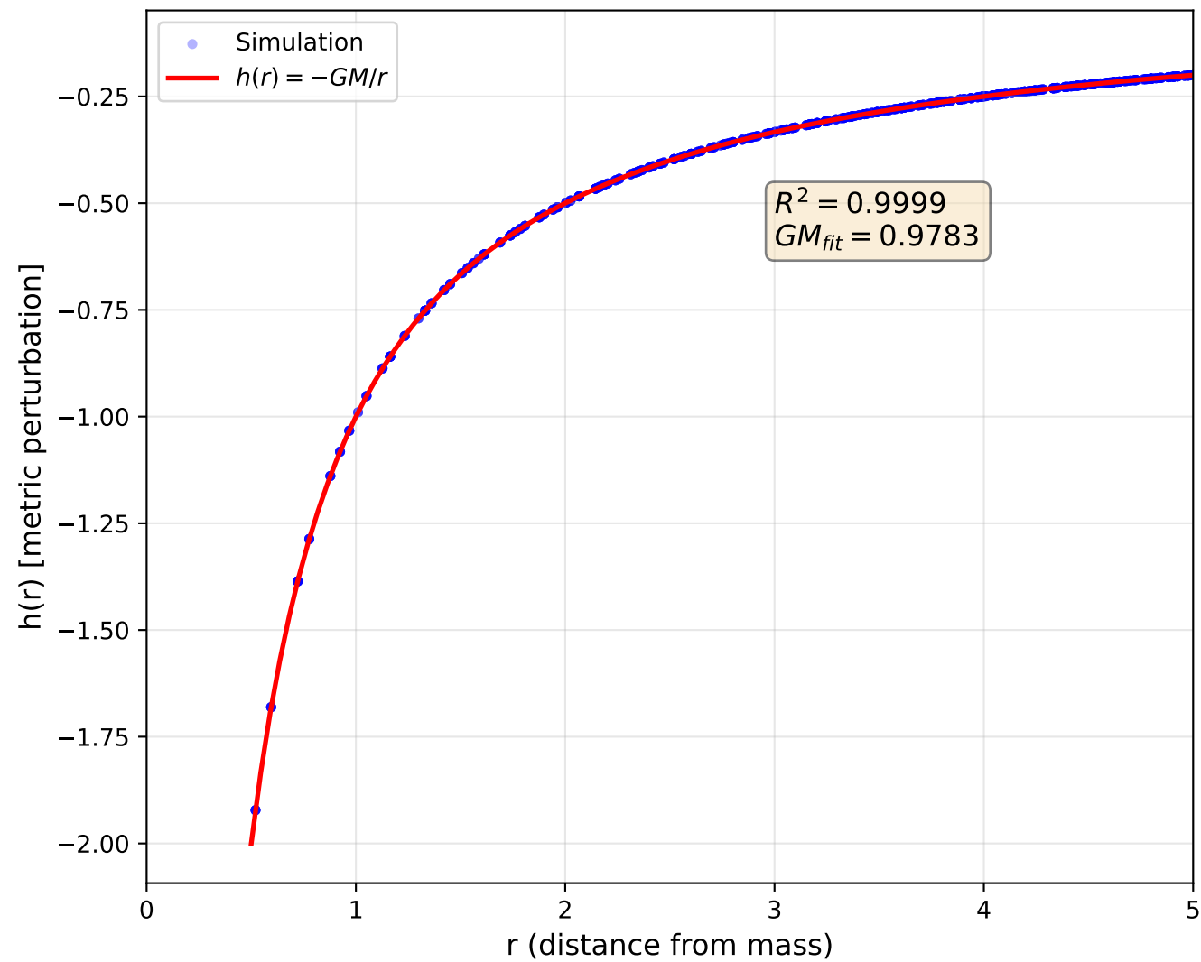
Radial Profile: Newtonian 1/r Confirmed ( R^2 = 0.9999 )
