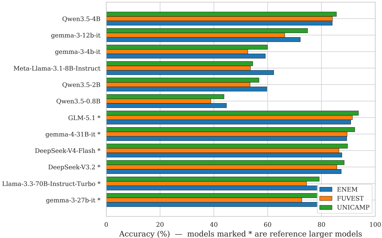
Accuracy across datasets
