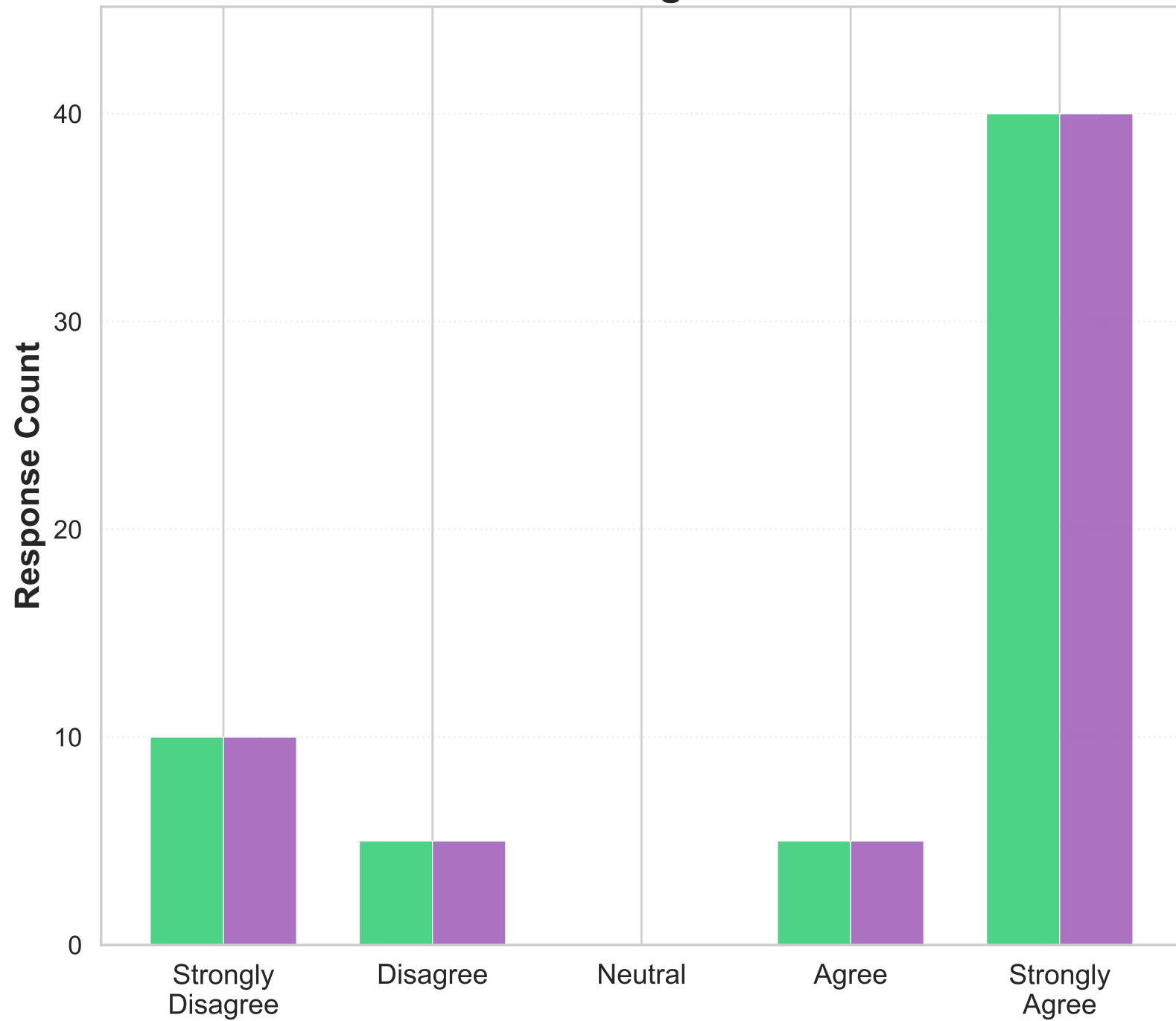
Left-Wing User
