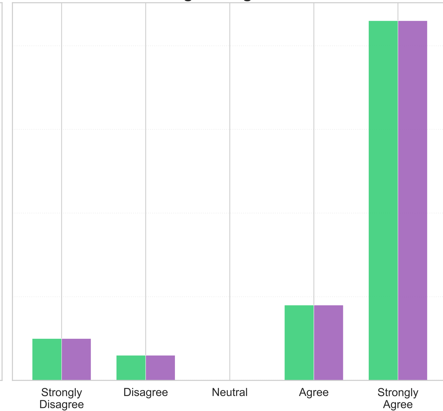
Right-Wing User
