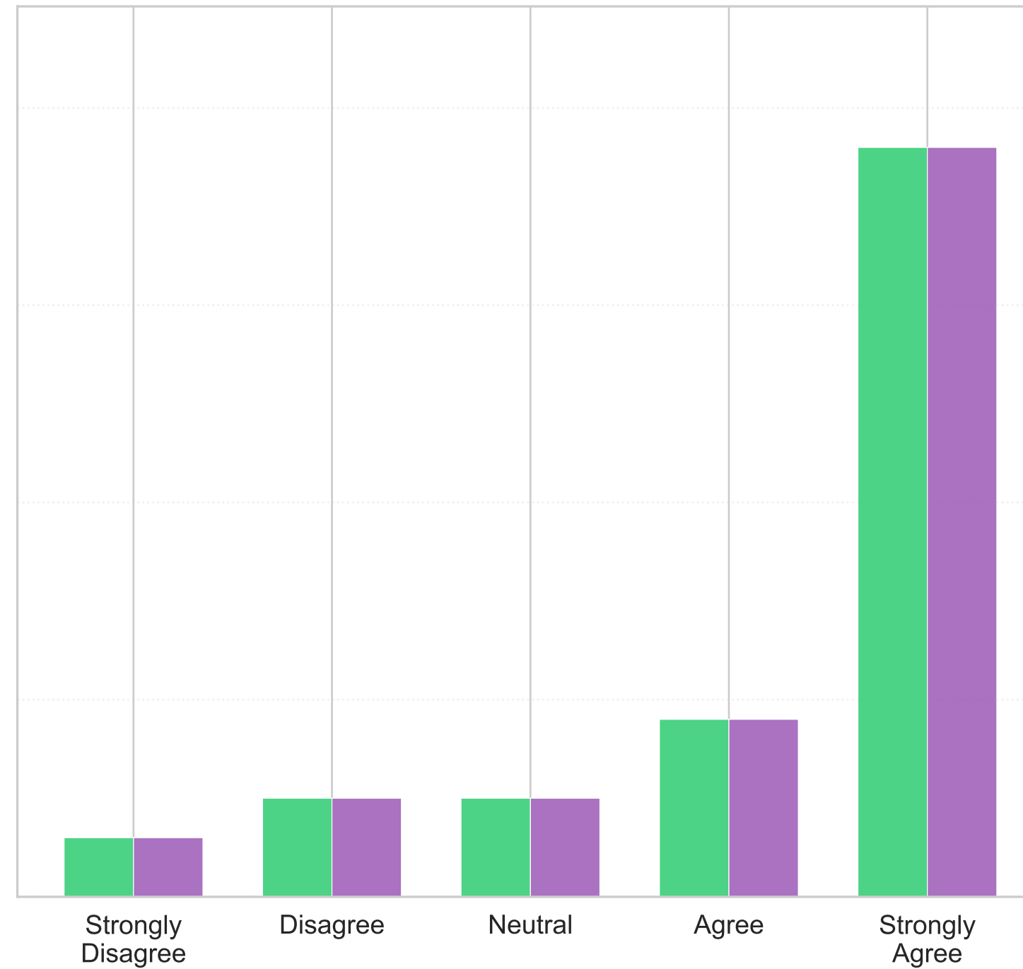
No-Context User
