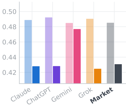
Brier score ↓
