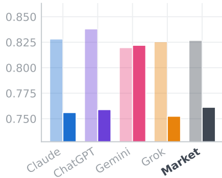
Log loss ↓
