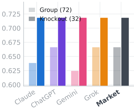
Accuracy ↑
