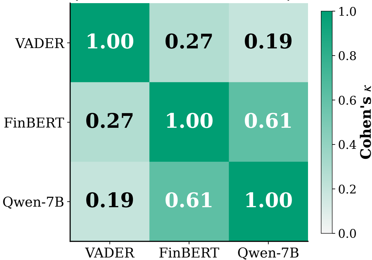
(a) Pairwise Cohen's \kappa (lower = more diverse)
