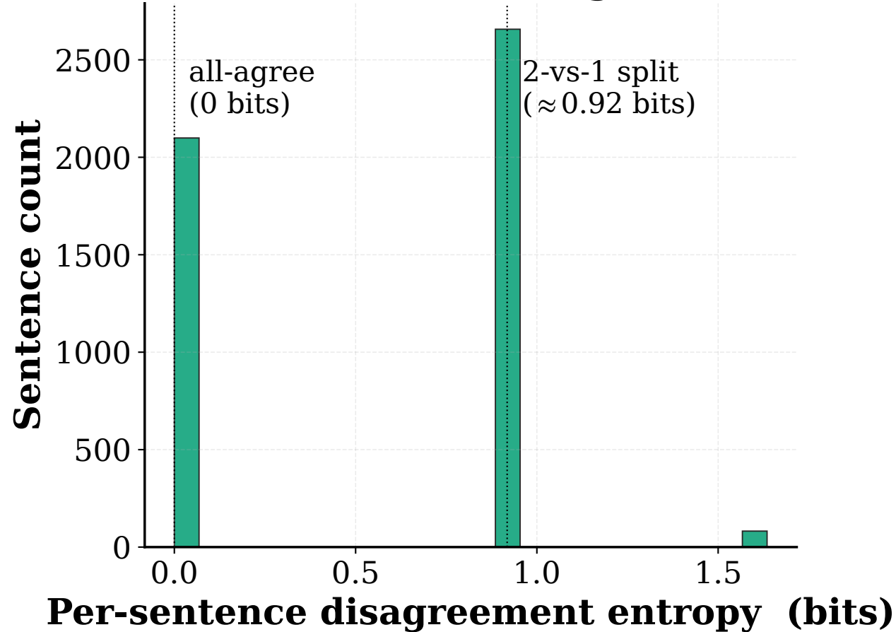
(b) Committee disagreement entropy
