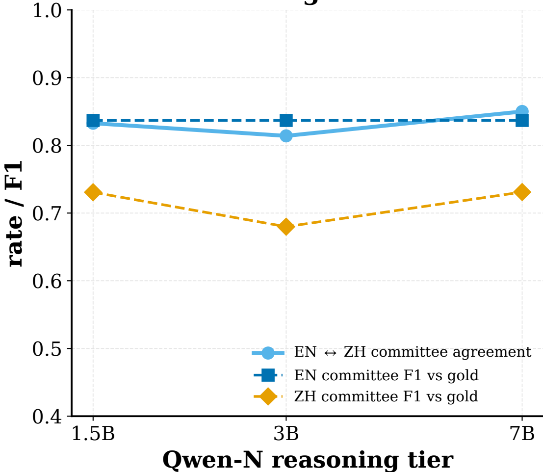
Naive cross-lingual committee
