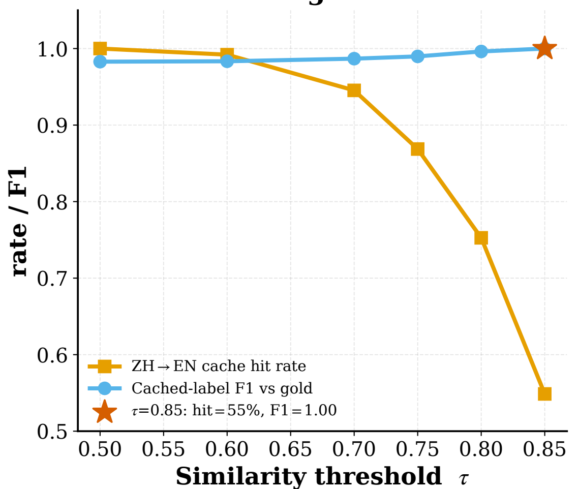
SCD as cross-lingual canonicalizer
