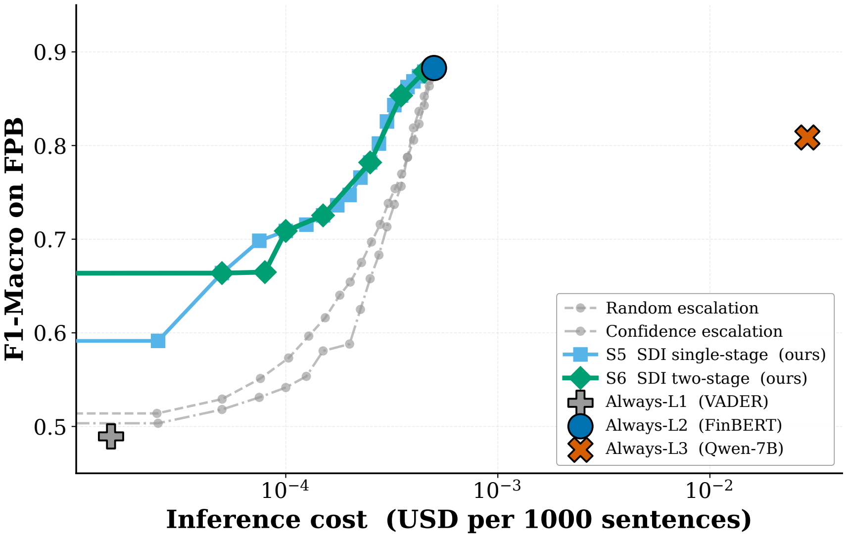
Token-economic Pareto frontier
