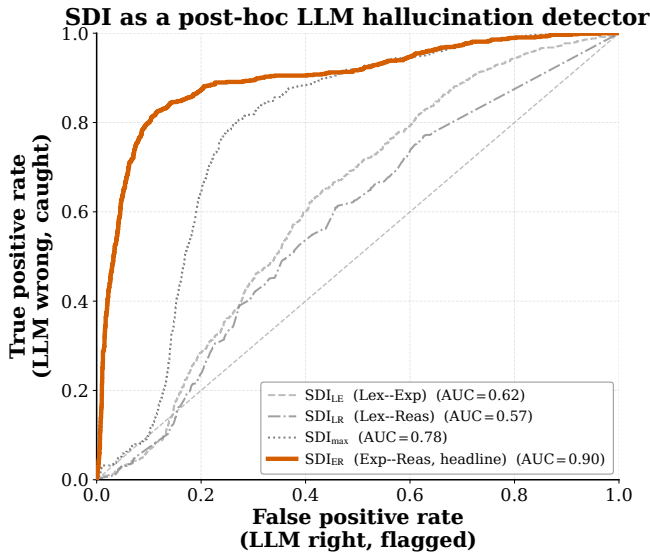
Figure 12: SDI as a post-hoc LLM-hallucination detector on FPB. SDI_{ER} (FinBERT vs. Qwen-7B) reaches AUC = 0.90 for the binary “LLM gives the wrong label” task.
