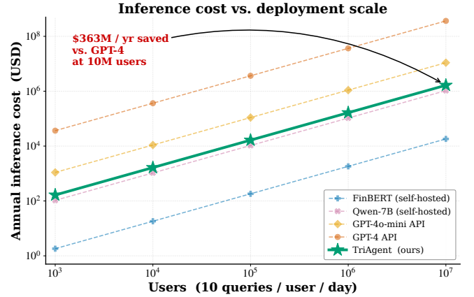
Figure 1: Annual inference cost vs. user count (10 queries/user/day). At 10 M users, default-to-cloud-LLM costs $11 M–$365 M/yr; TriAgent shaves this to $1.65 M/yr, a $9.3 M/yr saving against GPT-4o-mini.
