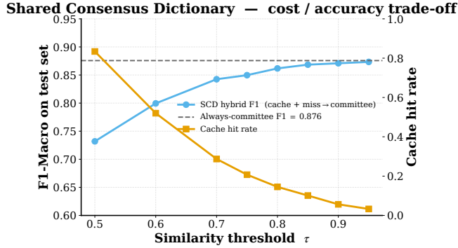
Figure 9: SCD accuracy / hit-rate trade-off as \tau varies. The deployable sweet spot is \tau \approx 0.85 . Production caches (orders of magnitude larger than our 3.4K-entry build set) would see substantially higher hit rates at the same \tau .
