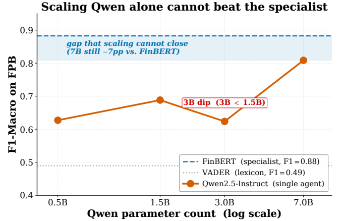
Figure 5: Single-agent F1 vs. Qwen size on FPB. The domain-specific FinBERT (dashed blue) outperforms every Qwen variant up to 7 B; 3 B underperforms 1.5 B (over-predicts neutral) and 14 B-4bit lands below 7 B-bf16 (quantisation cost exceeds the size gain).
