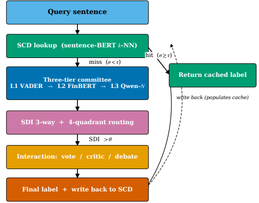
Figure 2: TriAgent system architecture. A query first hits the SCD; on cache miss the three-tier committee runs (VADER→FinBERT→Qwen-N), then SDI computation, then an interaction protocol when SDI exceeds threshold. The final committee label is written back into the SCD.
