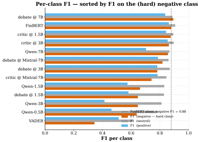
Figure 8: Per-class F1 sorted by F1 on the (hard) negative class. Debate@7B reaches 0.893 on negative — +1.4 pp over FinBERT alone (0.879), the only setting where any committee strategy beats the specialist on a class. The lift comes from precision improvement at near-equal recall.
