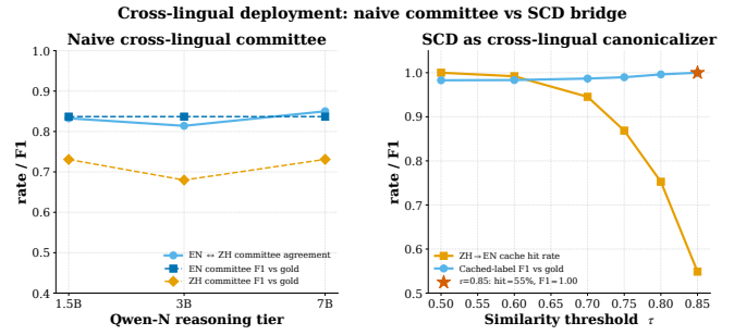
Figure 10: Cross-lingual deployment. Left : naive cross-lingual committees agree 81–85% with their English counterparts ( \kappa 0.55 –0.66). Right : the SCD acts as a cross-lingual canonicaliser — multilingual sentence-BERT lets a Chinese query find its English cached answer at hit-rate 0.95 / F1 0.99 for \tau = 0.70 .
