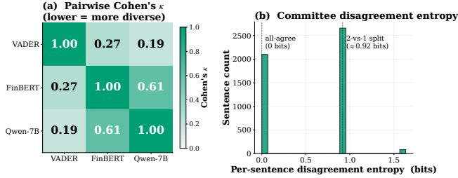
Figure 4: Pairwise Cohen’s \kappa (left) and per-sample disagreement entropy (right). Low \kappa confirms bias diversity; the bimodal entropy distribution shows the committee is either fully aligned or split 2-vs-1.
