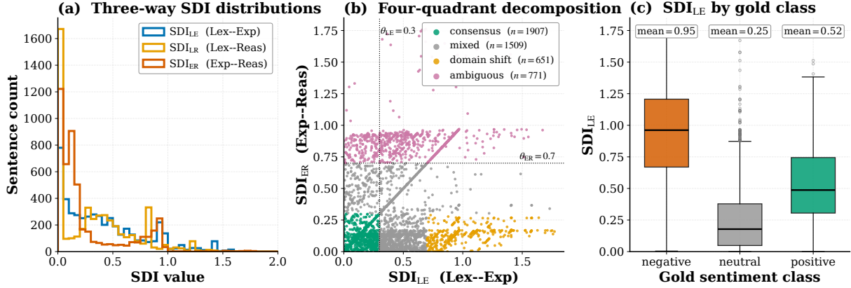
Figure 3: Three-way SDI on FPB. Left : distributions of the three pairwise SDIs. Centre : four-quadrant scatter of (\text{SDI}_{LE}, \text{SDI}_{ER}) . Right : \text{SDI}_{LE} by gold class — negative has highest mean disagreement (0.945; ANOVA F = 1777 , p < 10^{-200} ).
