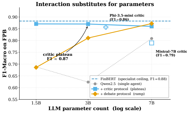
Figure 6: The paper’s central finding: interaction substitutes for parameters within a model family . Critic F1 plateaus at \approx 0.87 across Qwen-1.5B/3B/7B (sky-blue squares); debate ramps from 0.69 to 0.87 (orange diamonds); single-agent F1 stays well below in grey. Mistral-7B (hollow markers at the right) is family-specific lower.
