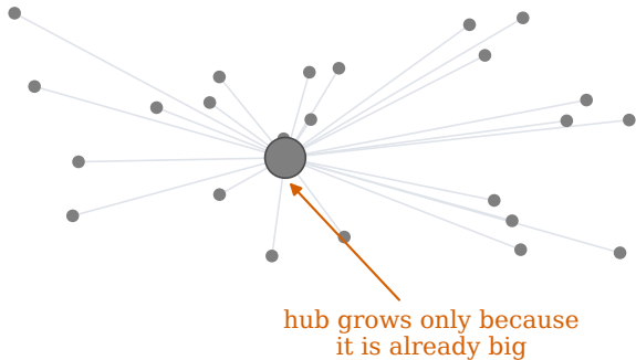
(a) preferential attachment (BA)
