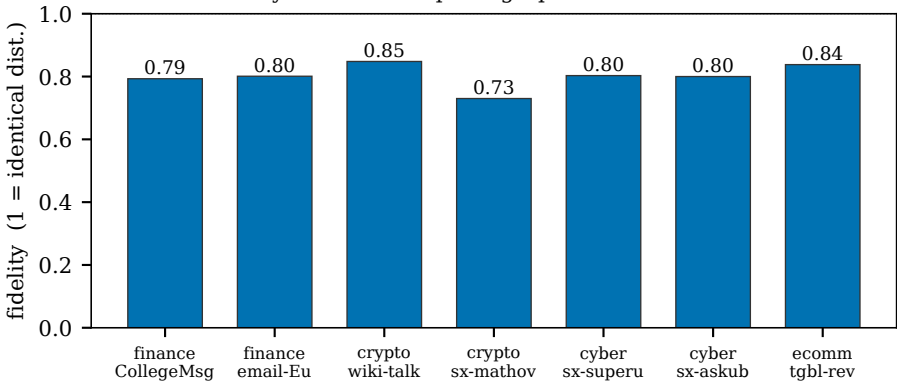
fidelity vs 7 real temporal graphs across 4 domains
