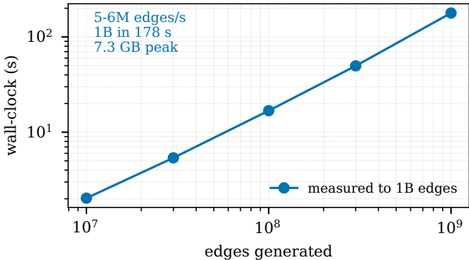
(a) generation time vs scale
