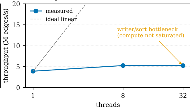
(b) plateaus at \sim 8 threads \rightarrow IO-bound
