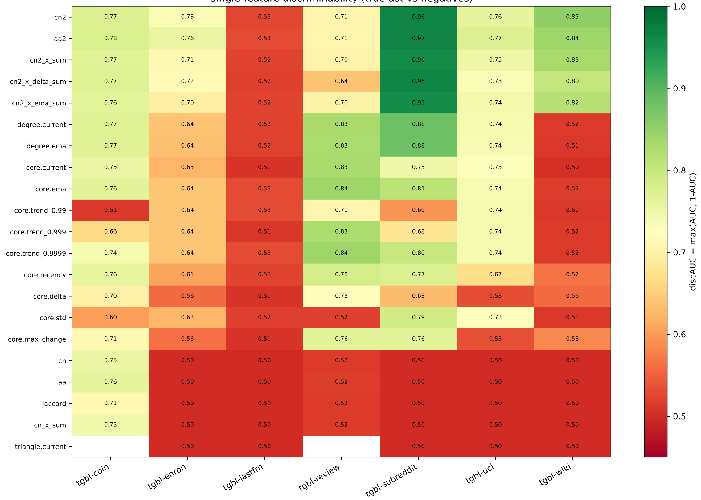
Single-feature discriminability (true dst vs negatives)
