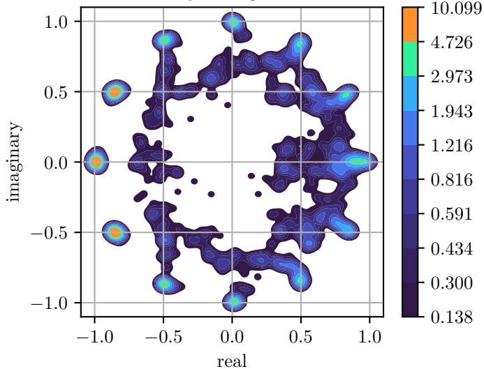
Density of eigenvalues
