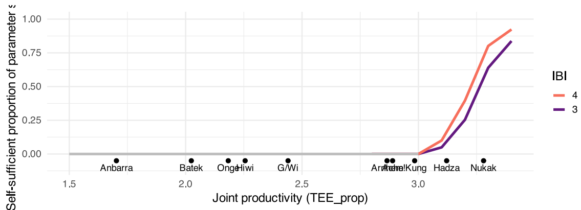
Figure S 9: The proportion of the parameter space in which family energy balance never falls below 0, and therefore does not need energy transfers from others, as a function of the joint production of the wife and husband.
