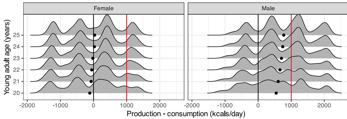
Figure S 10: Variation in net energy production of young adults due to variation in skill ontogeny parameters. The black dots represent the means of each distribution. The vertical red line represents the approximate TEE of an infant or very young child. The four modes are caused by the four sex-specific values of TEE_{prop} . Young adults' positive net energy production could help provision young siblings (helper-at-the-nest), or the siblings of one's spouse, e.g., brideservice.
