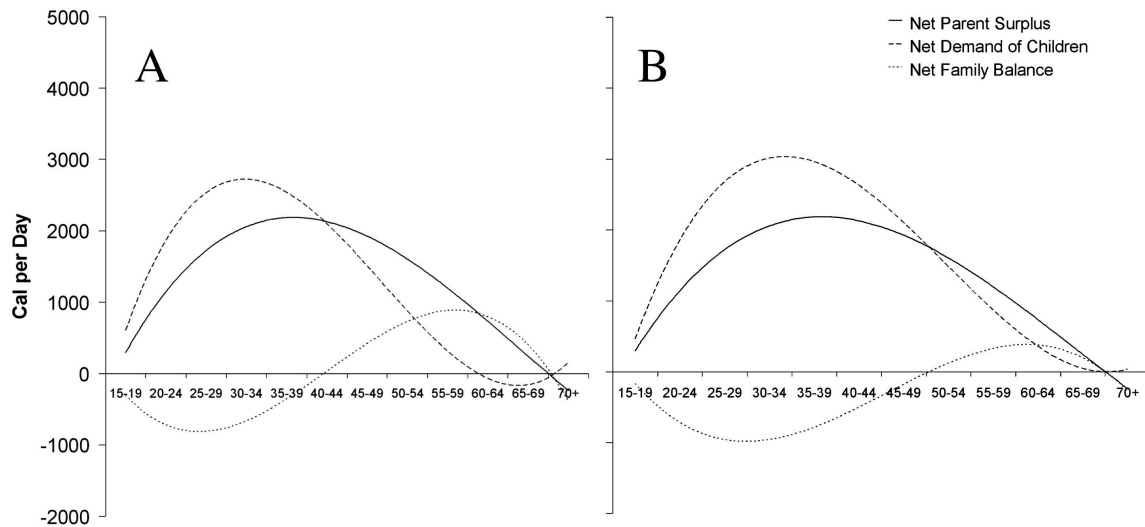
Figure S 4: A: Tsimane parental production, children's demands, and net family production. B: Simulated values based on delayed menopause. Figures from Kaplan et al. (2010).
