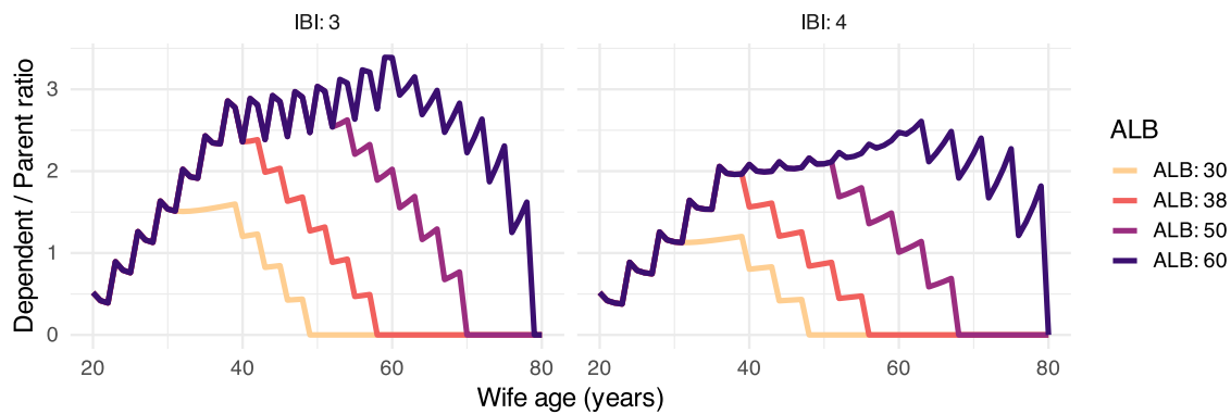
Figure S 12: Ratio of the number of dependents to the number of surviving parents for varying values of ALB, IBI, and wife's age.
