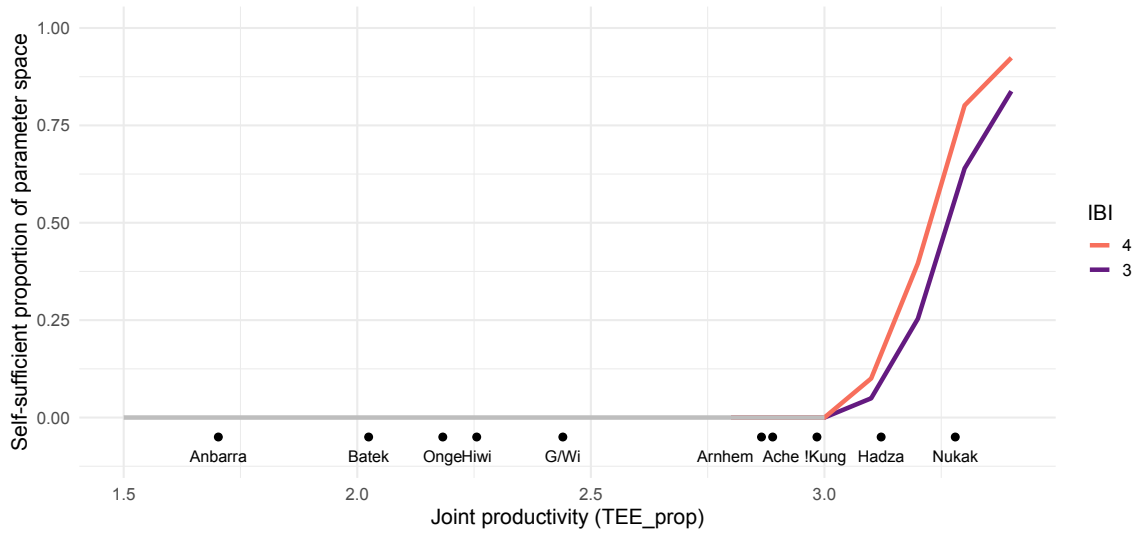
Figure S 10: The proportion of the parameter space in which family energy balance never falls below 0, and therefore does not need energy transfers from others, as a function of the joint production of the wife and husband.
