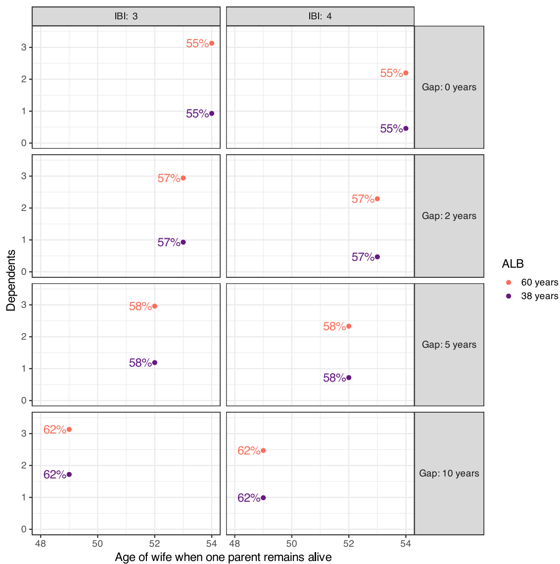
Figure S 13: The number of dependents when, on average, only one parent remains alive due to wife and husband mortality. Gap is the age gap in marriage. Percentage values are the probabilities that the one remaining parent is the wife.
