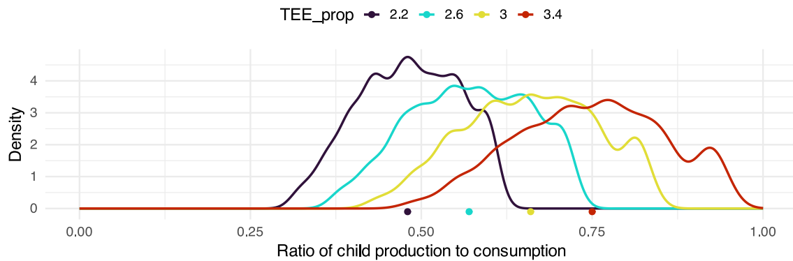
Figure S 7: Distribution of child production / consumption ratios across the lifecourse for different values of TEE prop . Dots along the x-axis are the mean values of each distribution.
