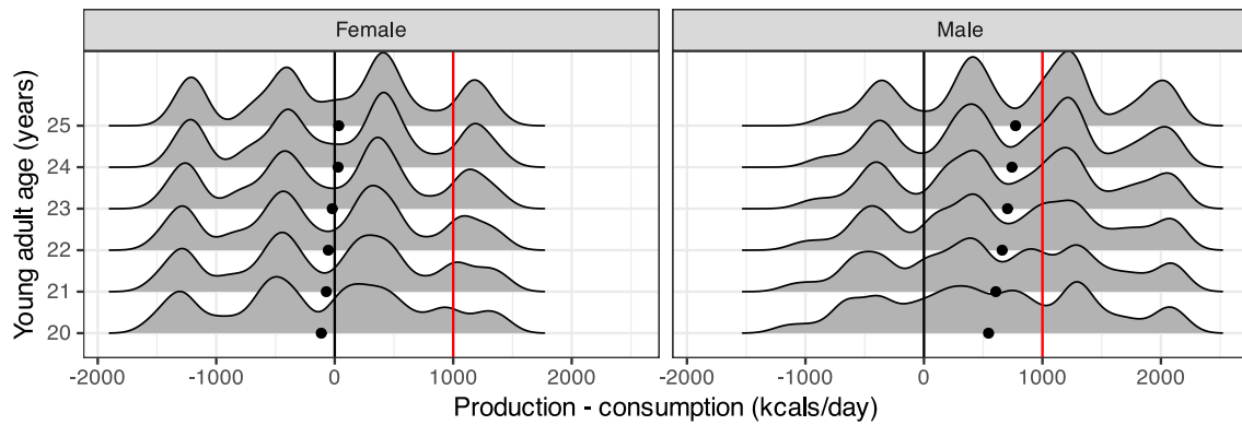
Figure S 11: Variation in net energy production of young adults due to variation in skill ontogeny parameters. The black dots represent the means of each distribution. The vertical red line represents the approximate TEE of an infant or very young child. The four modes are caused by the four sex-specific values of TEE_{prop} . Young adults' positive net energy production could help provision young siblings (helper-at-the-nest), or the siblings of one's spouse, e.g., brideservice.
