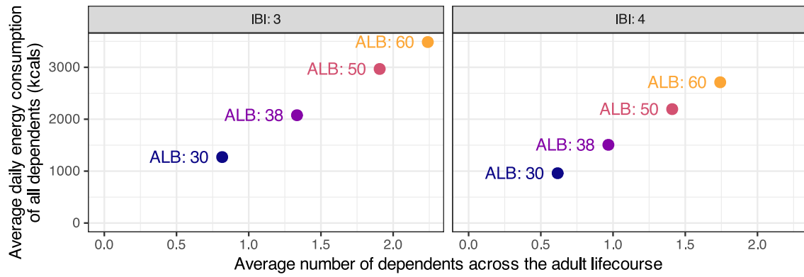
Figure S 8: Average number and daily energy consumption of dependents that families were supporting each day across the adult lifespan, for each value of the ALB and IBI.
