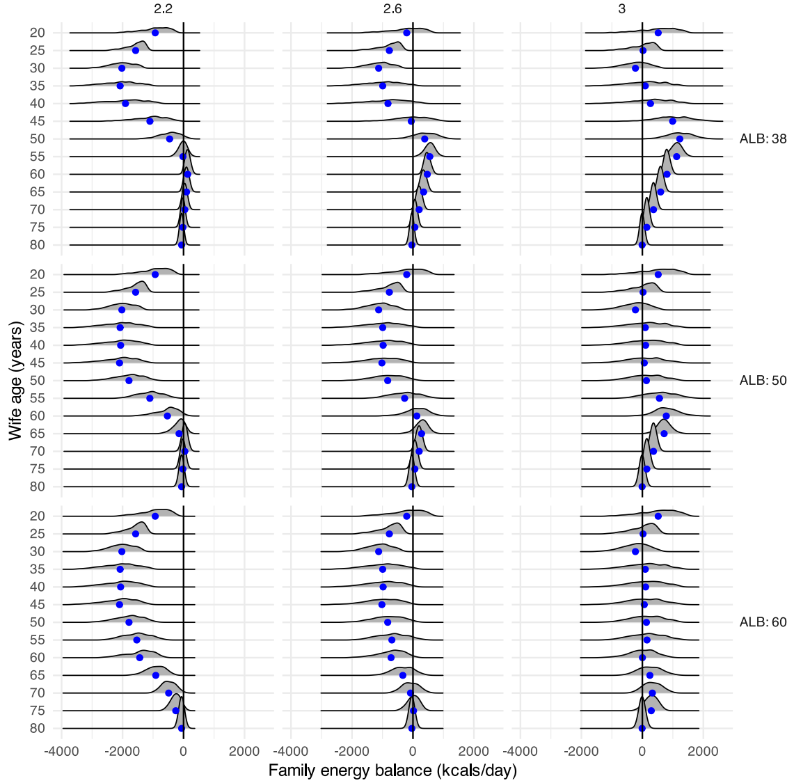
Figure S 9: Variation in energy balance at each age due to variation in skill ontogeny parameters and IBI. Columns: joint adult productivity as a proportion of adult TEE ( TEE_{prop,f} + TEE_{prop,m} ). Rows: ages of last birth (ALB). Blue dots are the mean values. Joint productivity and ALB restricted to intermediate values for clarity.
