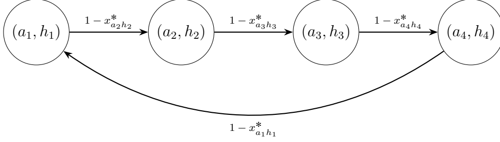
Figure 3.1: A directed cycle in the auxiliary graph used for separation. Each vertex is an assignment pair (a_i, h_i) . The edge from (a_i, h_i) to (a_j, h_j) has weight 1 - x_{a_j h_j}^* .
