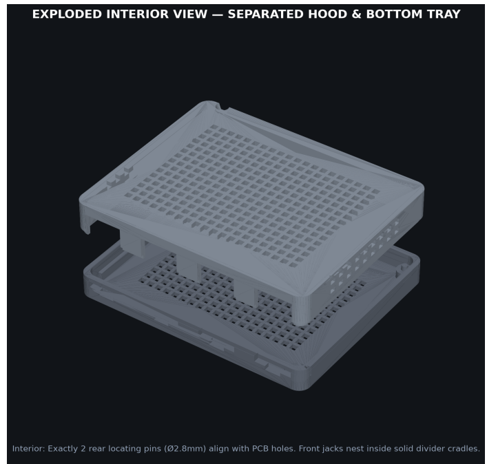
EXPLODED CLAMSHELL VIEW
