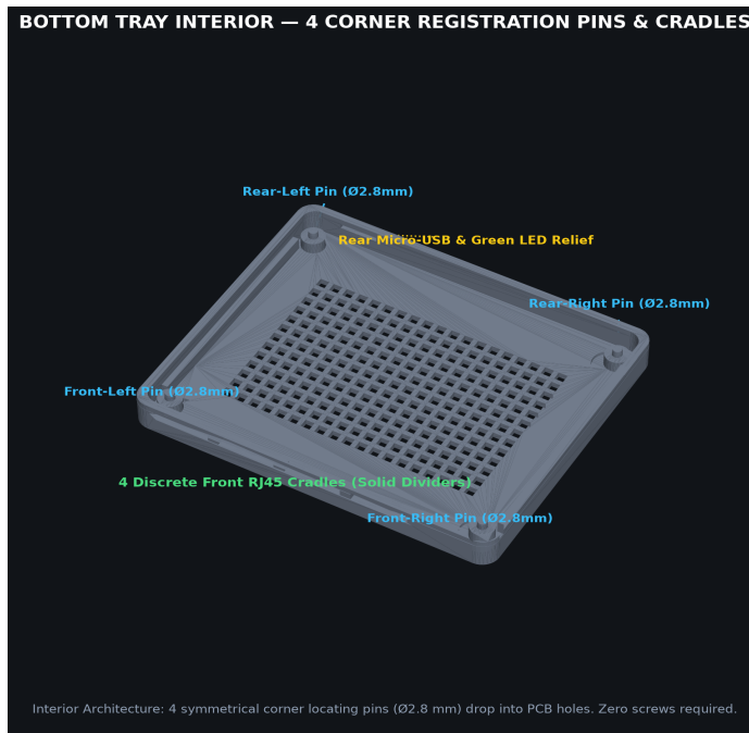
BOTTOM TRAY INTERIOR
