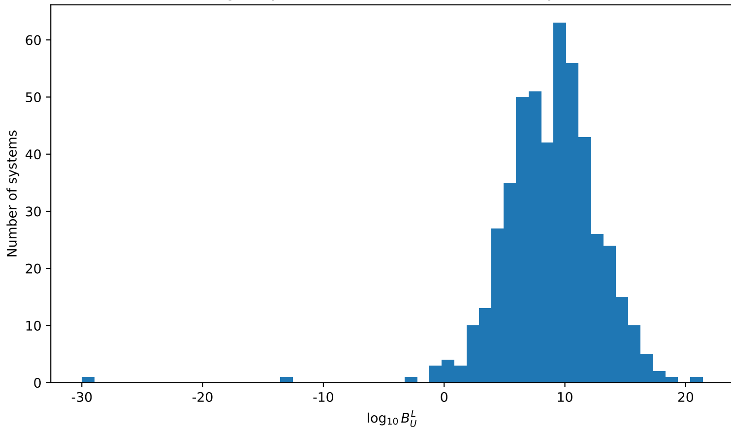
3-image Bayes Factors for Simulated Lensed Systems
