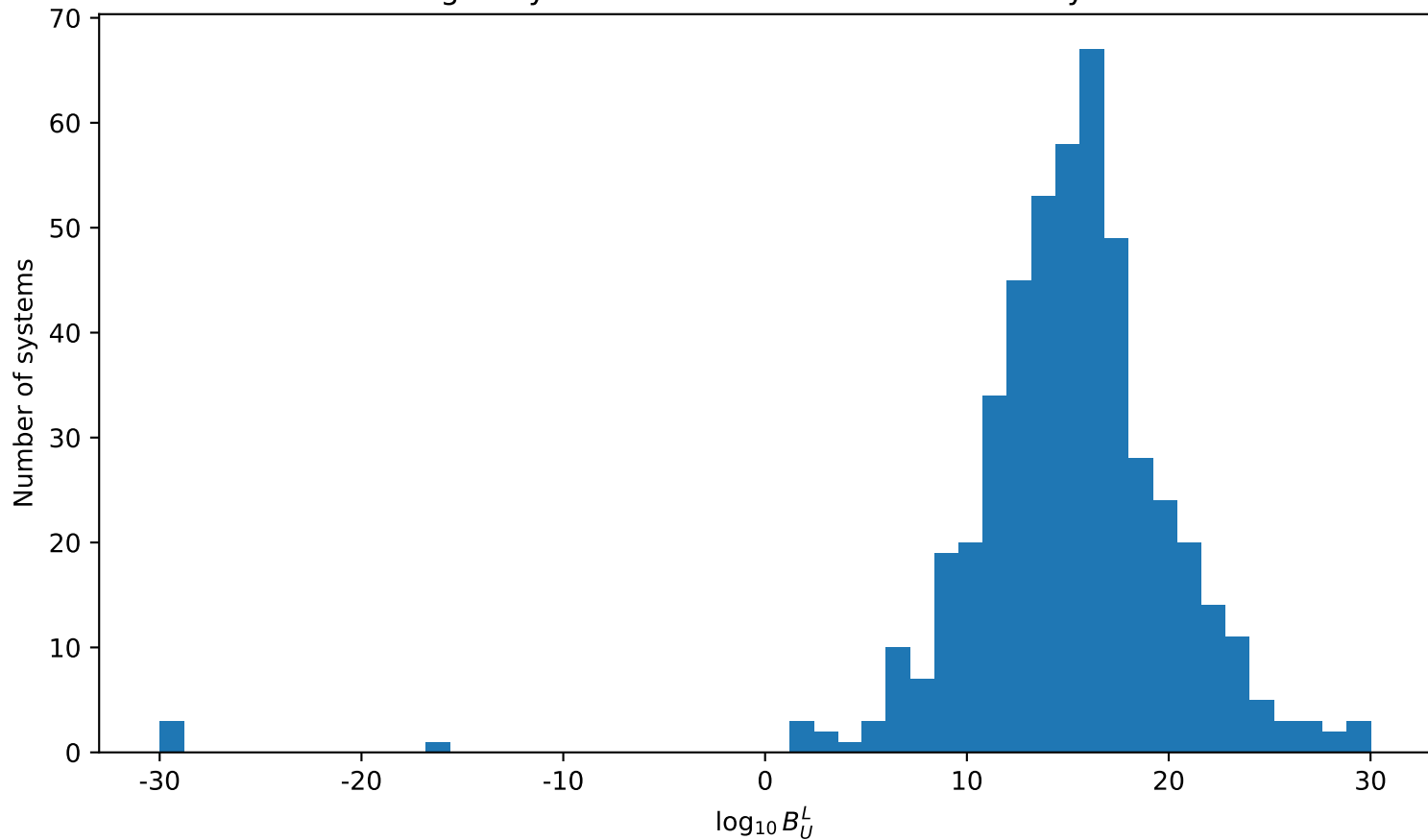
4-image Bayes Factors for Simulated Lensed Systems
