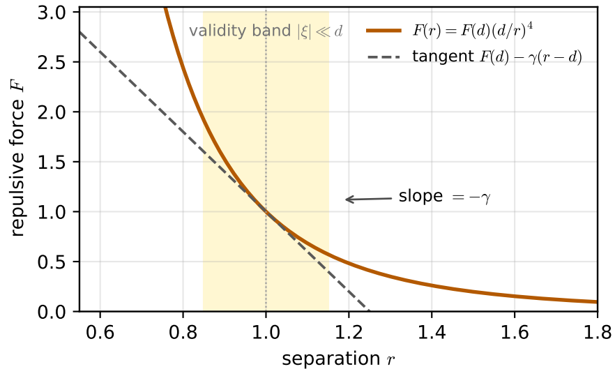
F(r) convex: tangent slope defines the magnetic stiffness
