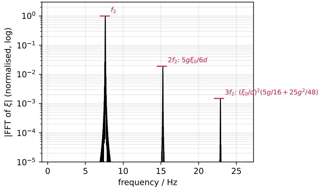
(b) harmonics of \xi = x_2 - x_1 : d = 24.5 mm, \xi_0 = 4.2 mm, undamped
