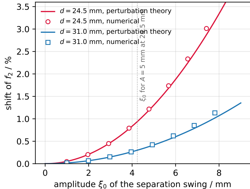
(a) amplitude dependence of f_2
