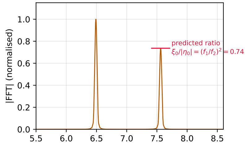
(b) spectra of the 45 s records
