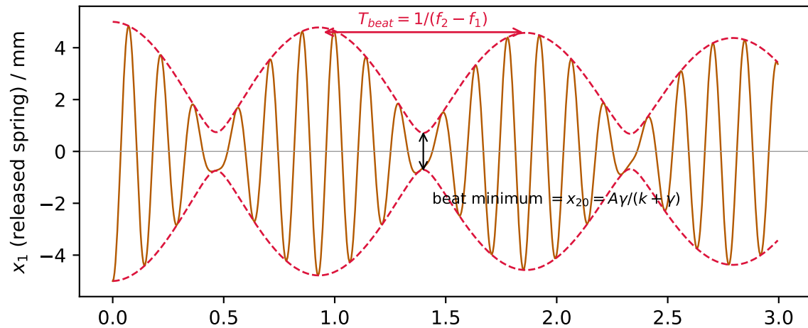
(a) d = 24.5 mm, A = 5 mm, \tau_d = 21 s: f_1 = 6.49 , f_2 = 7.56 Hz
