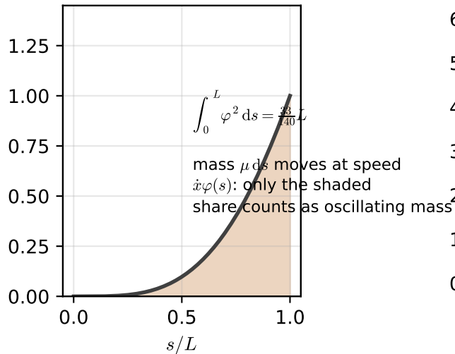
where the moving mass is ( \propto \varphi^2 )
