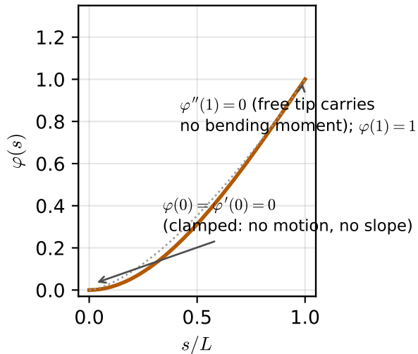
deflection shape y(s, t) = x(t) \varphi(s)
