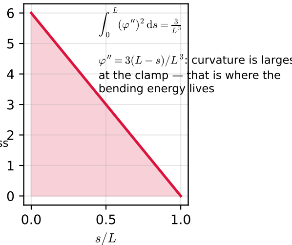
where the bending is ( \propto \varphi''^2 )
